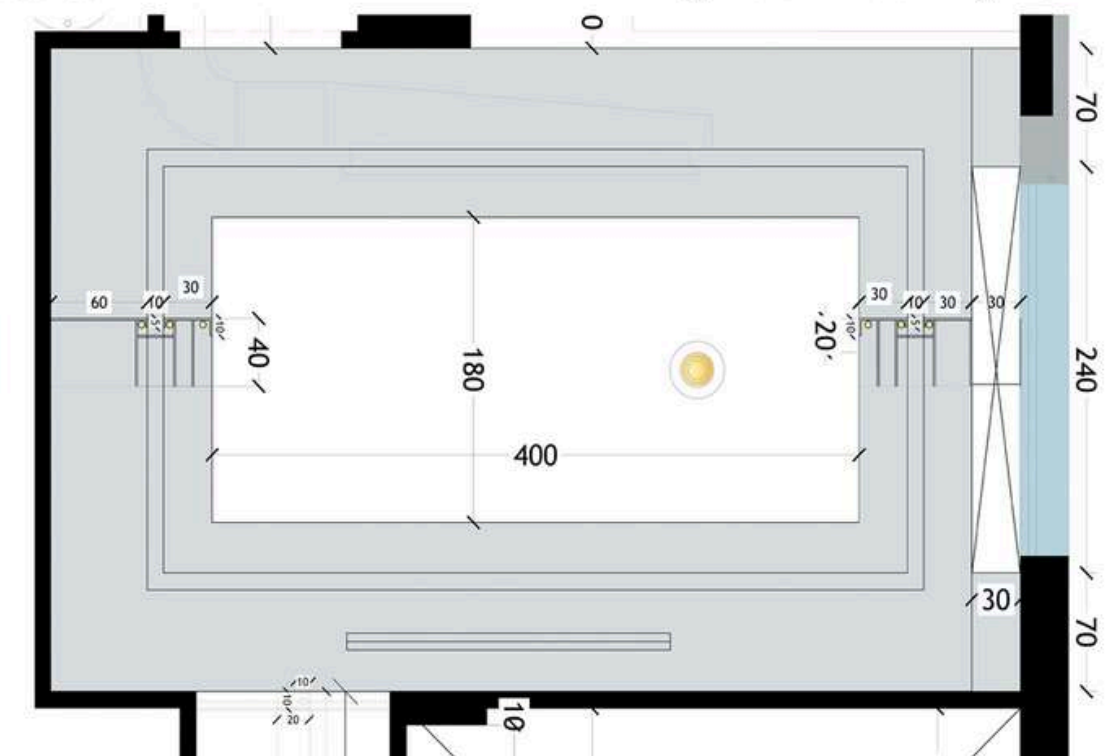
Living Room - Ceiling Plan
