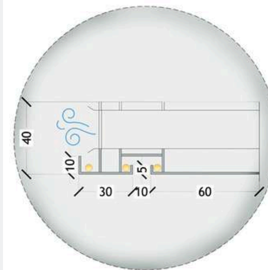
Ceiling Detail
